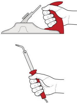
Figure 28 Select tools that can be held with a neutral wrist or in a handshake position with the hand adopting a comfortable, not too open or too closed, grip. Orient jigs and fixtures holding the work piece, so the wrist does not have to bend.
