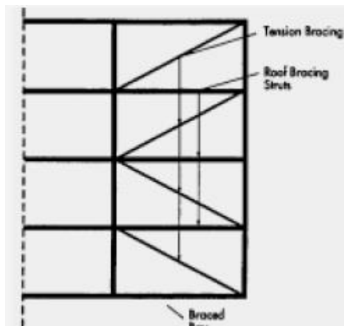
Figure A8. Roof tension bracing
