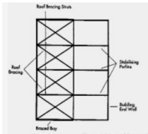
Figure A10. Building end wall
