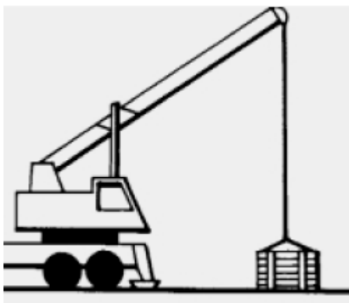
Figure 8. Correct slinging
