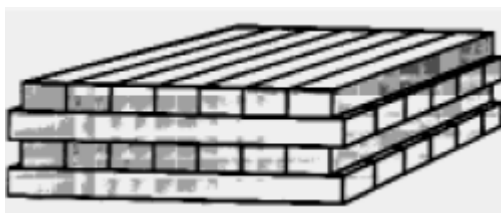
Figure 7. 'Pigsty' configuration
