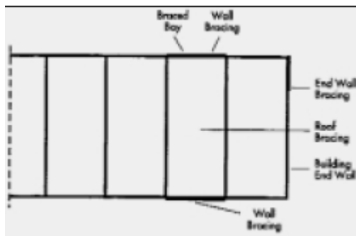
Figure A2. Alternative wall bracing location
