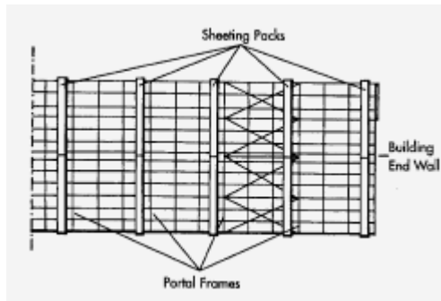
Figure A15. Location of sheeting packs.
