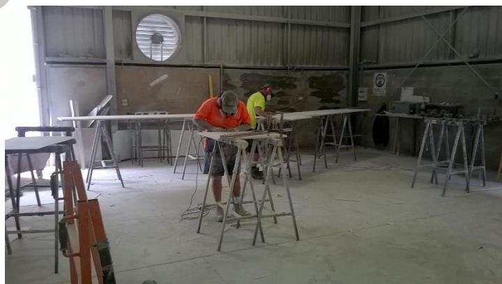
Figure 3 - Photo of two workers conducting dry cutting. Dust is visible on the floor and workers clothing. Enforcement action was taken to prohibit the process until exposure risks were managed. Photo by WHSQ.
