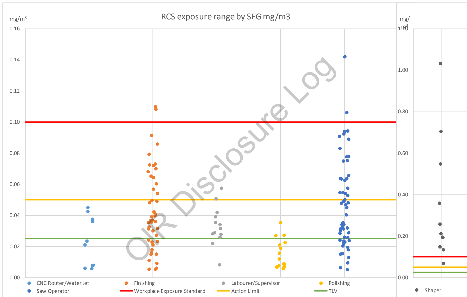
Figure 6 - Graph of individual exposures (8hr TWA) for each SEG
