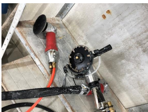
Figure 2 - Photo of a pneumatic polisher and grinder with water feeds.
