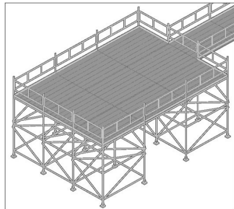
Figure 11 Birdcage scaffold 3
