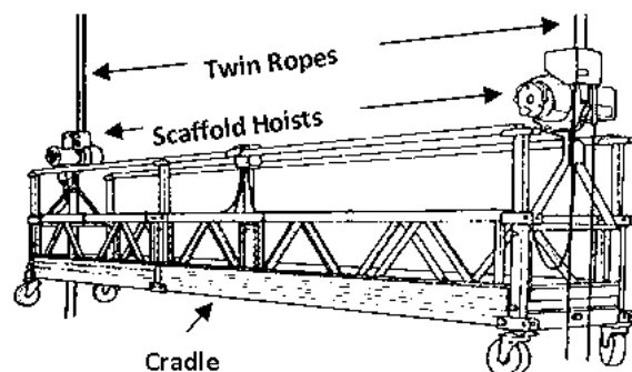
Figure 15b. Suspended (swing-stage) scaffold – Cradle (suspended) end
