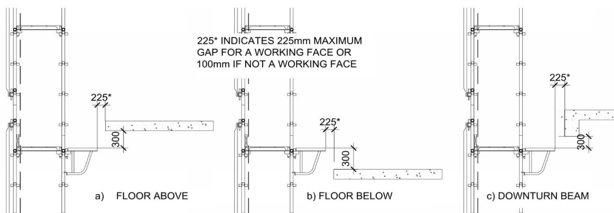
Figure 8 Allowable gaps
