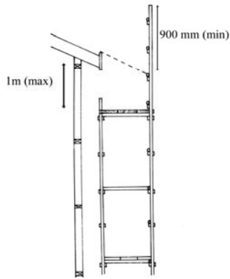
Figure 7a Fall arresting platform \leq 26^\circ
