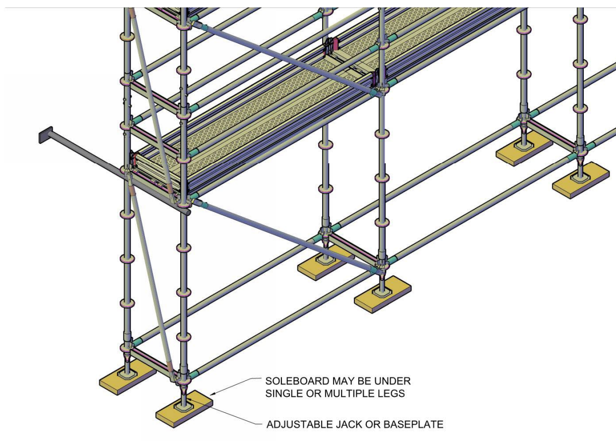
Figure 2. Soleboards and baseplates
