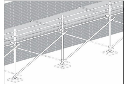
Figure 14 Single pole scaffold 5
