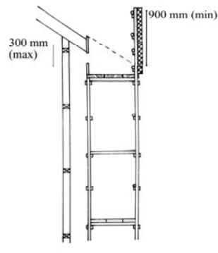
Figure 7b Fall arresting platform > 26^\circ
