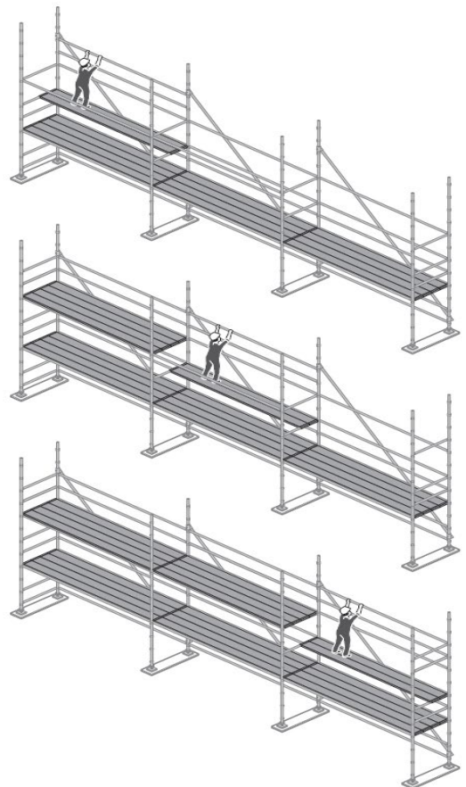
Figure 10 Scaffold erection 2
