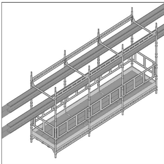
Figure 13 Hung scaffold 4
