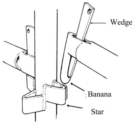
Figure 6. Mixing components. Avoid mixing different modular systems. Often connection points known as the 'star' and 'banana' used on these systems are of a different shape and tolerance and are not compatible.
