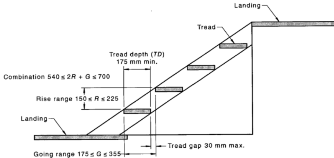
Figure 5. Temporary stairway configuration
