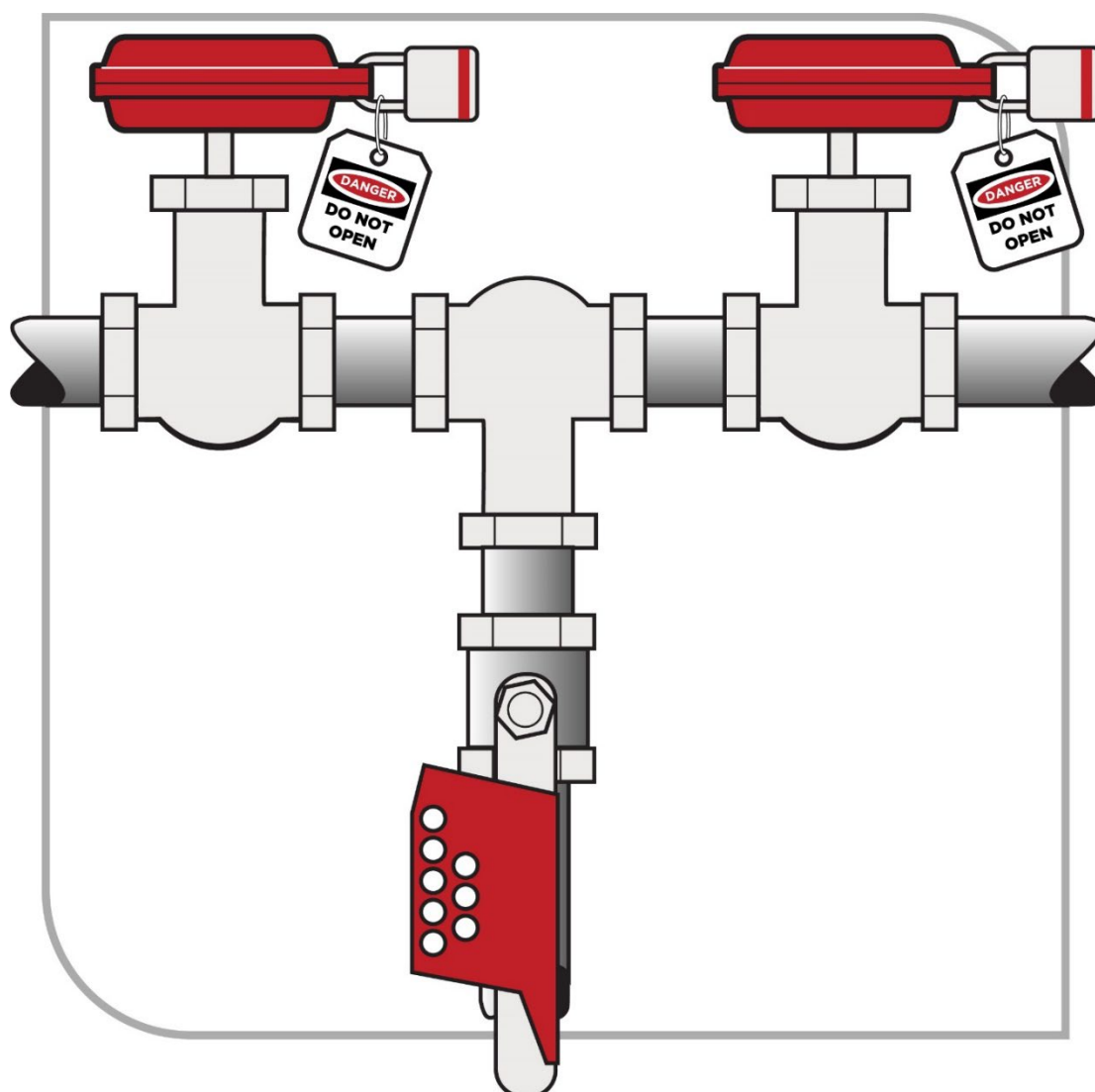
Figure 7 - Closing, locking and tagging at least two valves
