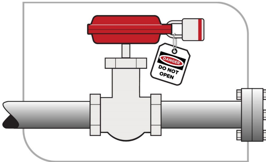
Figure 5 - Open end of pipe capped with the nearest valve closed, locked and tagged
