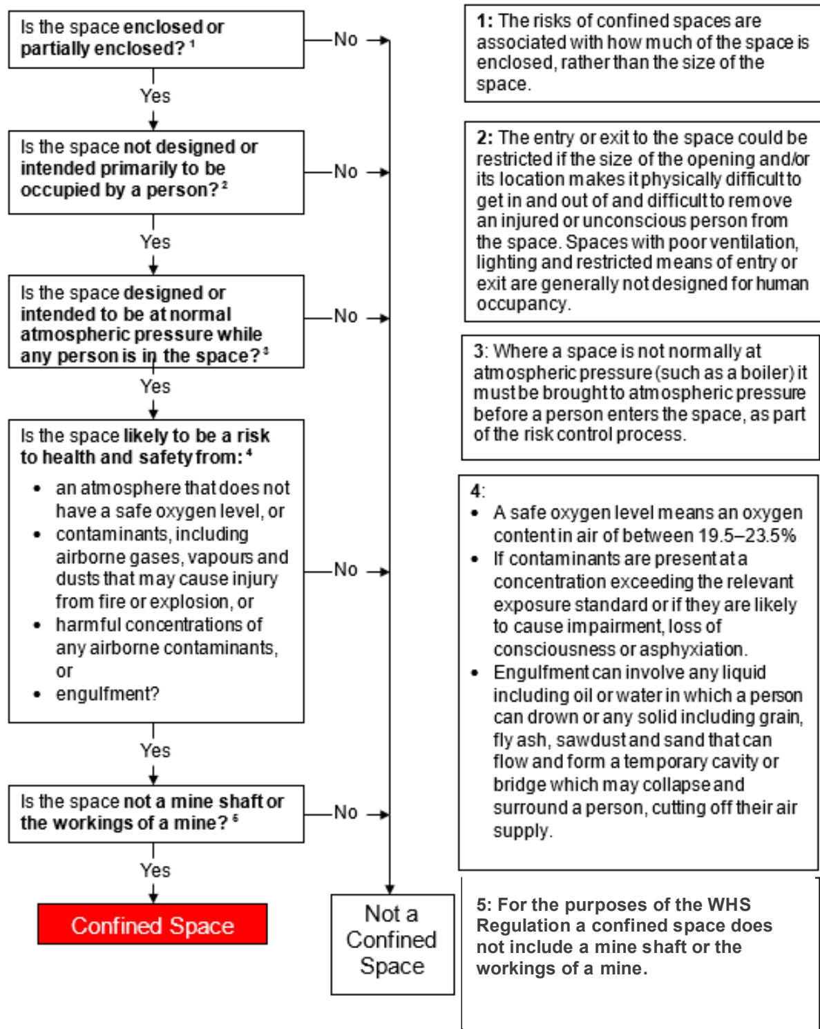
Figure 1 - How to determine whether a space is a confined space
