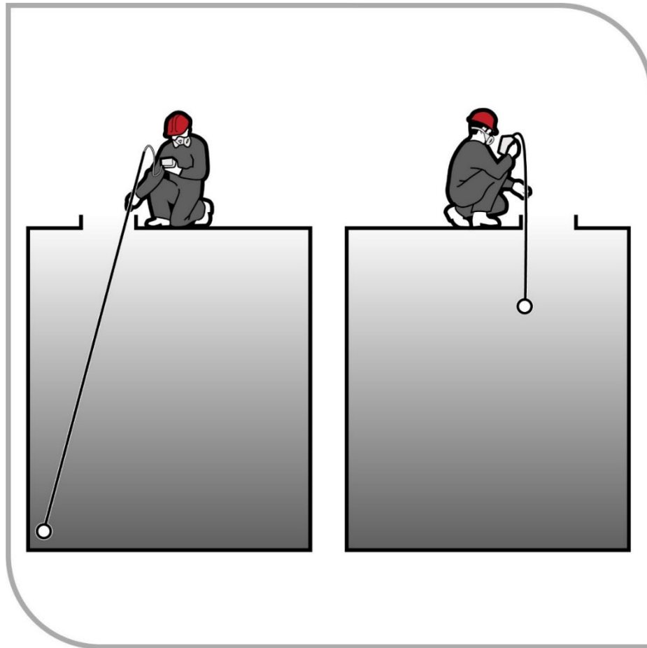
Figure 3 – Atmospheric testing of remote regions and different levels within the confined space
